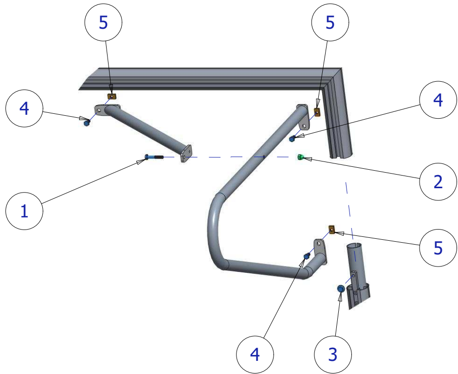
DETAIL A
